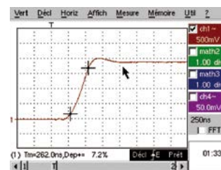
Pulse response
