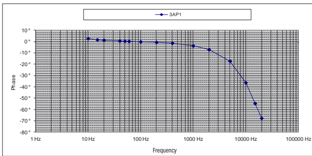
Typical phase shift according to frequency for a current of 2 A
