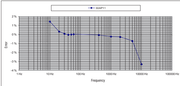
Typical error on measurement according to frequency for a current of 2 A
