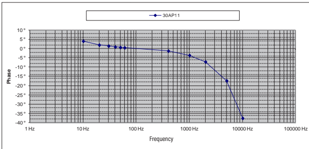
Typical phase shift according to frequency for a current of 2 A
