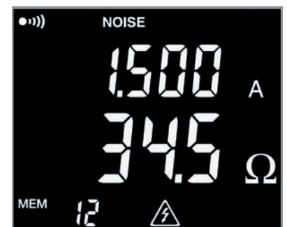
The Ground Voltage function is active whatever the measurement mode (standard or advanced).
